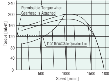
5RK60RGU(A)-AWU/ES01
