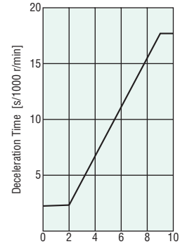
Deceleration Time Potentiometer Scale - Speed characteristics (Representative Values)
